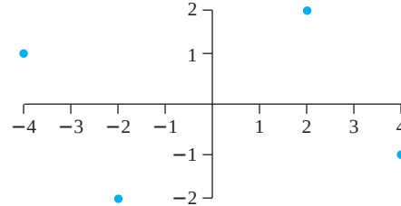
Figure 5.5 The population of pairs for Example 5.18
