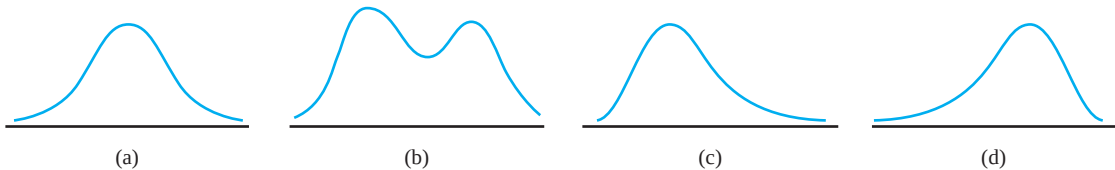
Figure 1.12 Smoothed histograms: (a) symmetric unimodal; (b) bimodal; (c) positively skewed; and (d) negatively skewed
