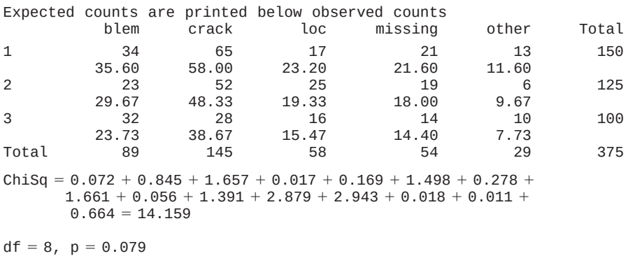
Figure 14.4 Minitab output for the chi-squared test of Example 14.13
