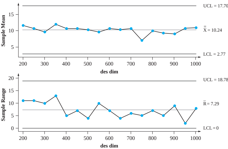
Figure 16.4 Control charts for the deviation-from-target data of Example 16.5 ■
